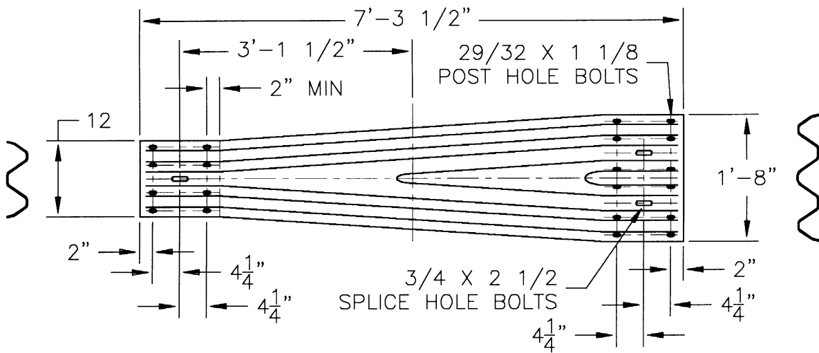
12GA/W-THRIE BEAM TRANSITION SECTION
