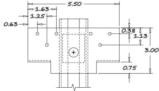
LINE BRACKET
