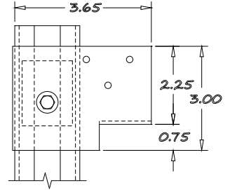
CORNER BRACKET
